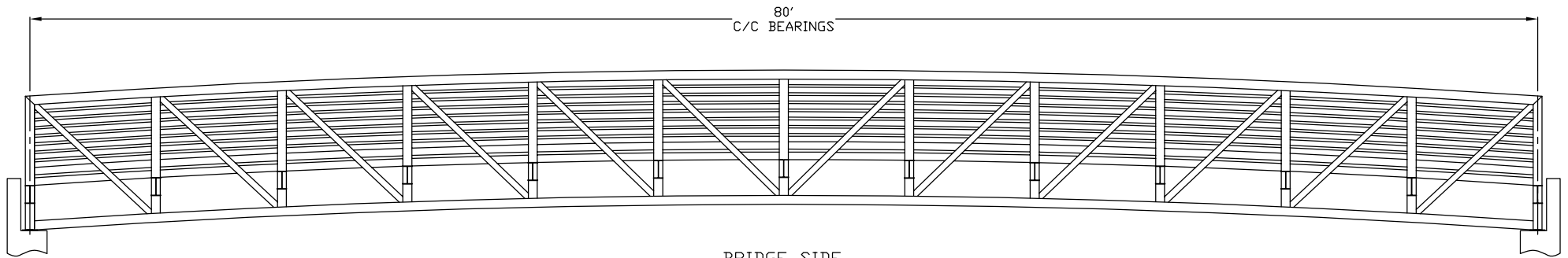
BRIDGE SIDE ELEVATION VIEW
