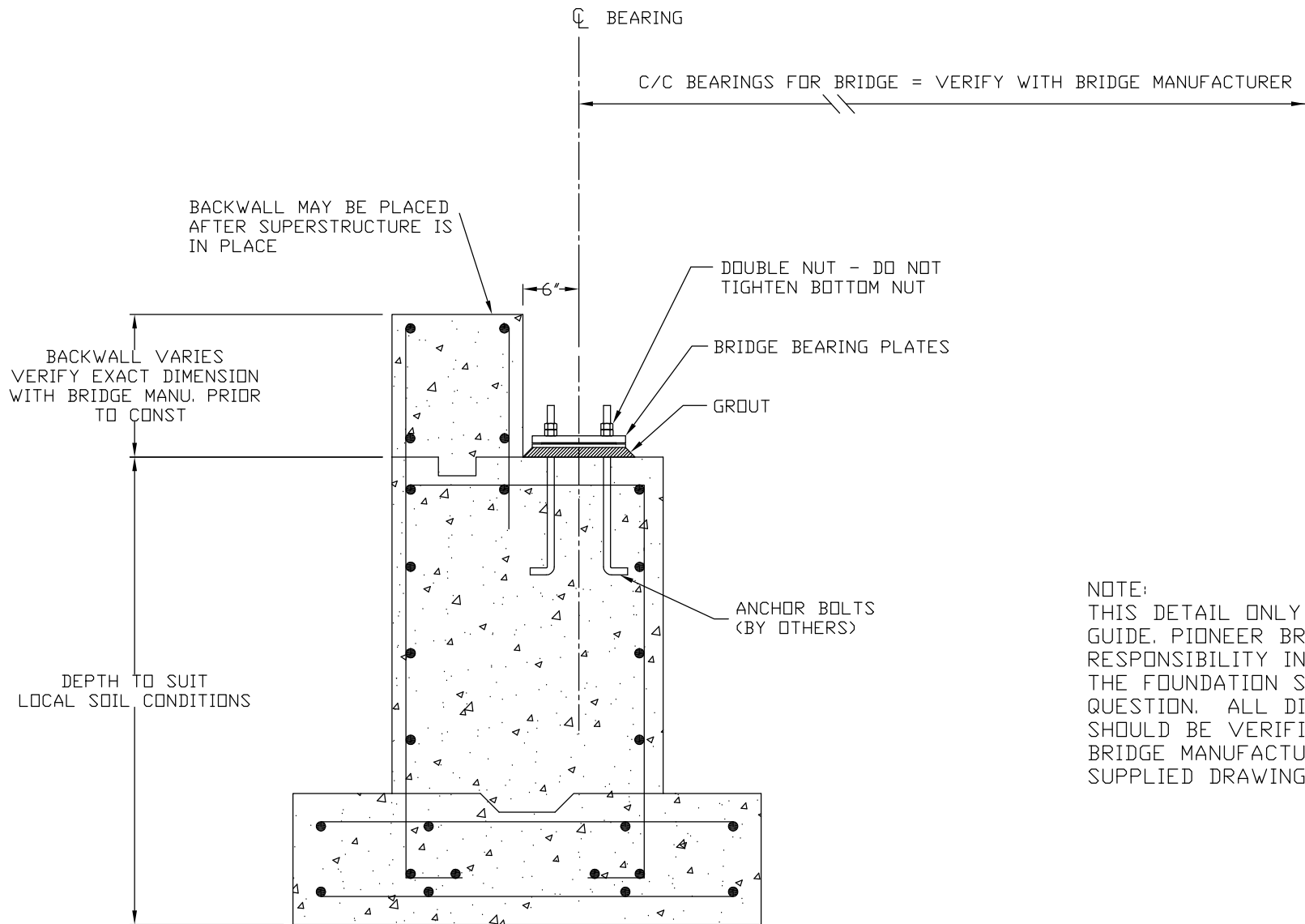
TYPICAL ABUTMENT CROSS SECTION
