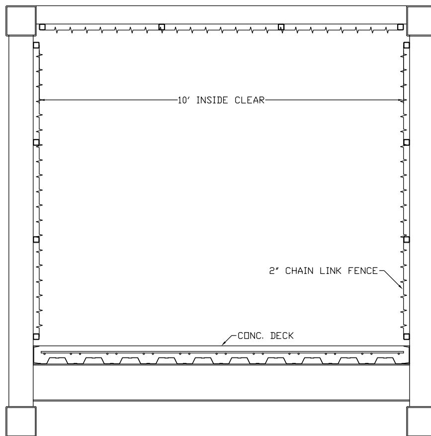
BRIDGE CROSS SECTION
