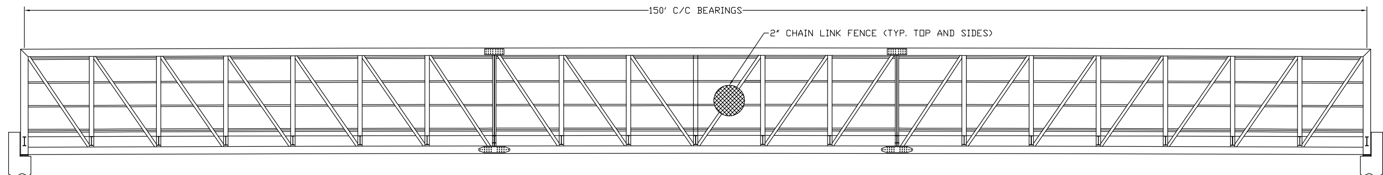
BRIDGE SIDE ELEVATION VIEW
