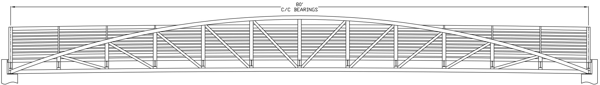
BRIDGE SIDE ELEVATION VIEW
