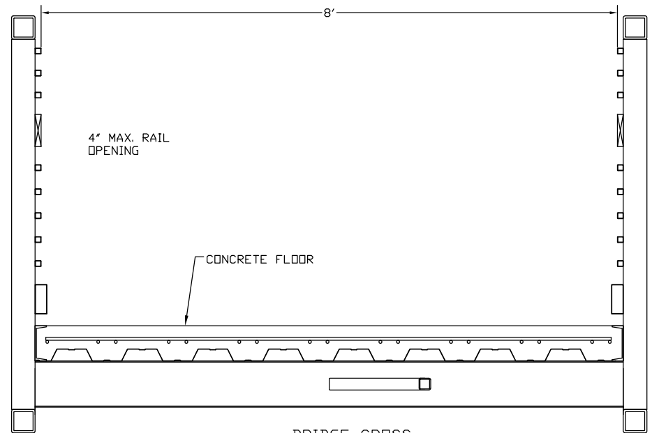
BRIDGE CROSS SECTION
