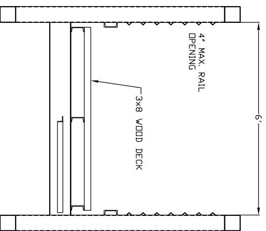
BRIDGE CROSS SECTION
